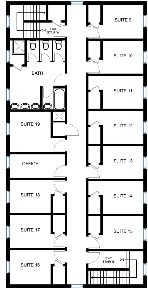
SECOND FLOOR
